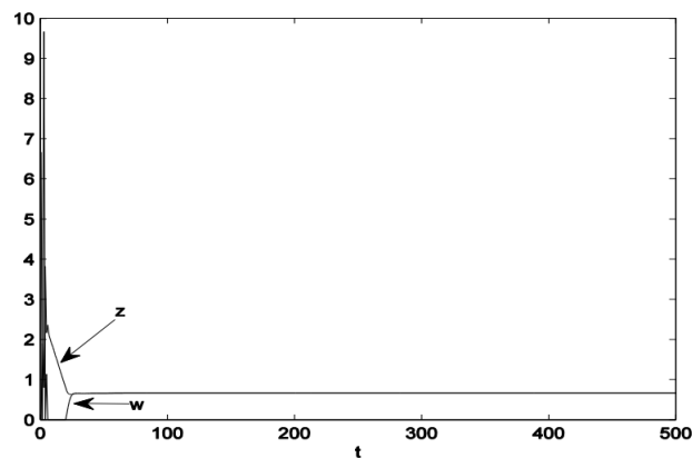
Figure 1: Optimal value of the LSIP in Example 1
