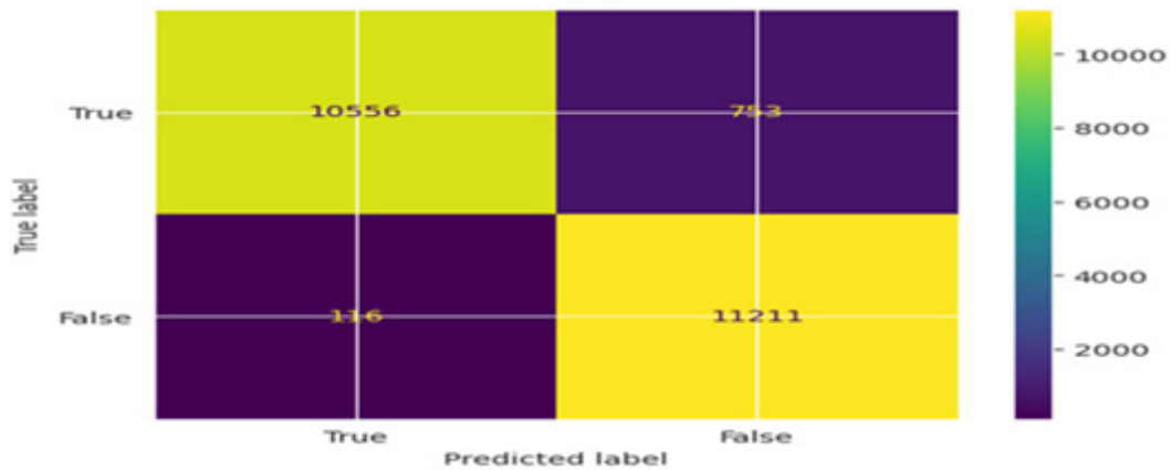
Figure 9: Confusion Matrix for LR Classifier for Notebook Features in 2024
