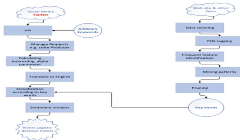
Figure 3: First stage of proposed framework
